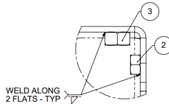
DETAIL J SCALE 1 : 1
